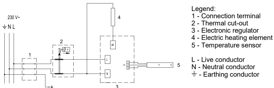
Fig. 4: Electric installation
