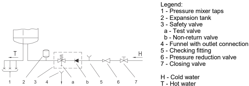
Fig. 2: Closed (pressure) system
