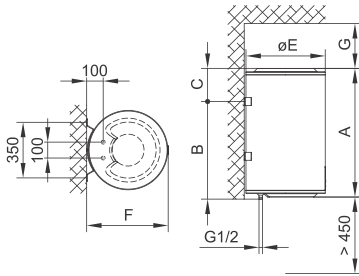
Fig. 1: Vertical installation on a wall
